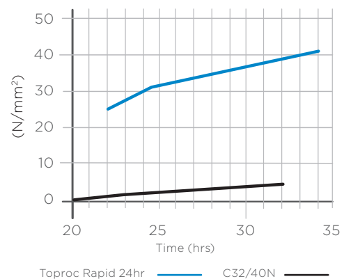
TYPICAL STRENGTH DEVELOPMENT OF TOPROC RAPID 24HR
