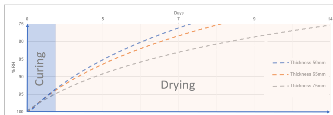
Chart 1: Typical drying times at 23°C and 50% relative humidity.
